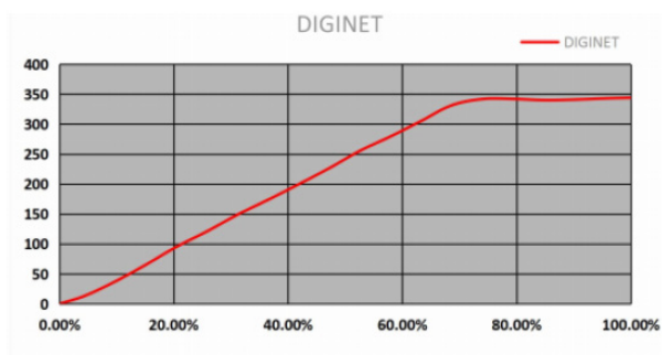
Fig 1: Dimming Curve with MEDM Diginet
